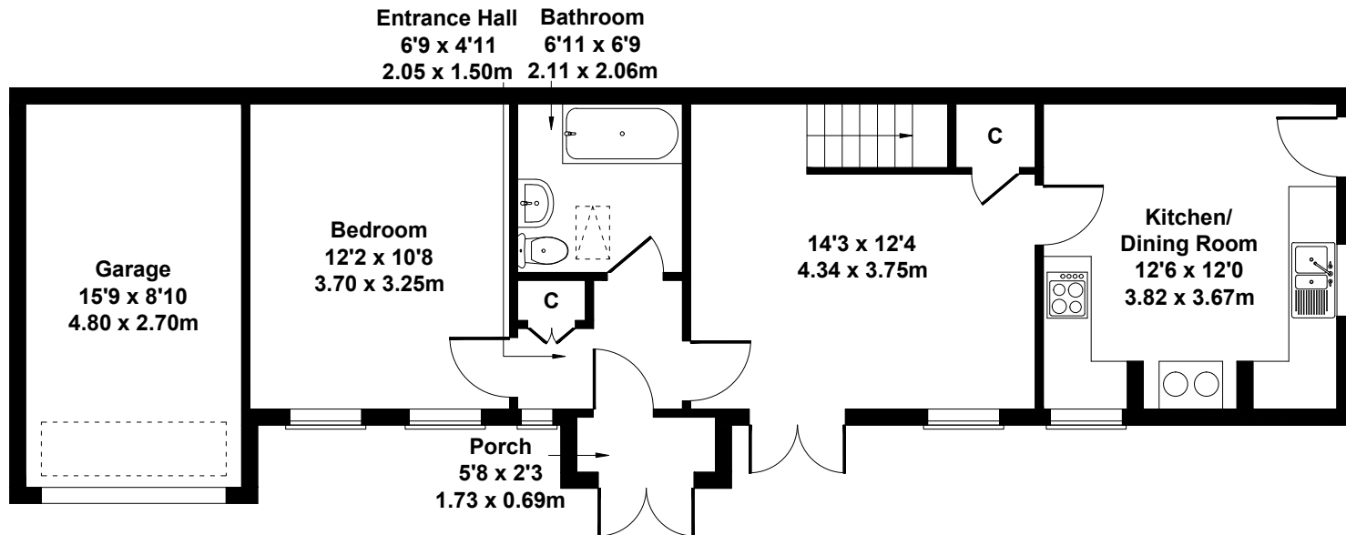
GROUND FLOOR
